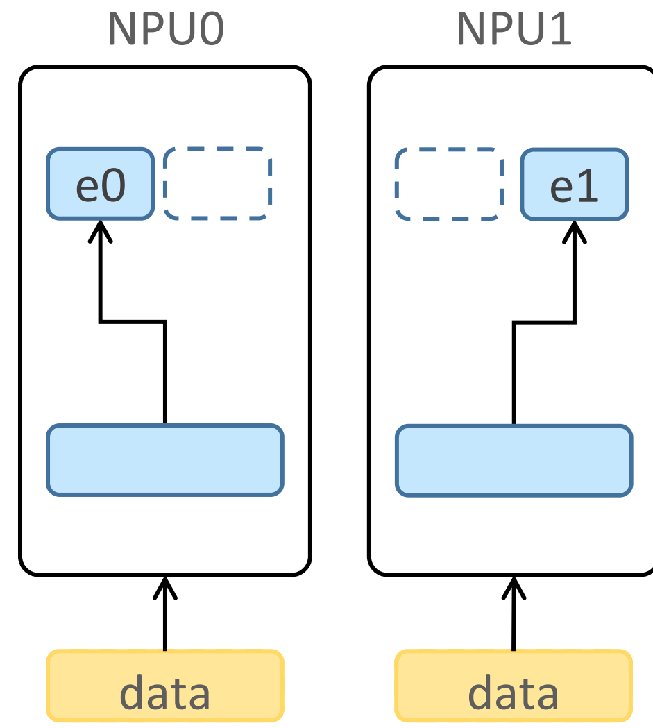
专家并行 expert parallel
